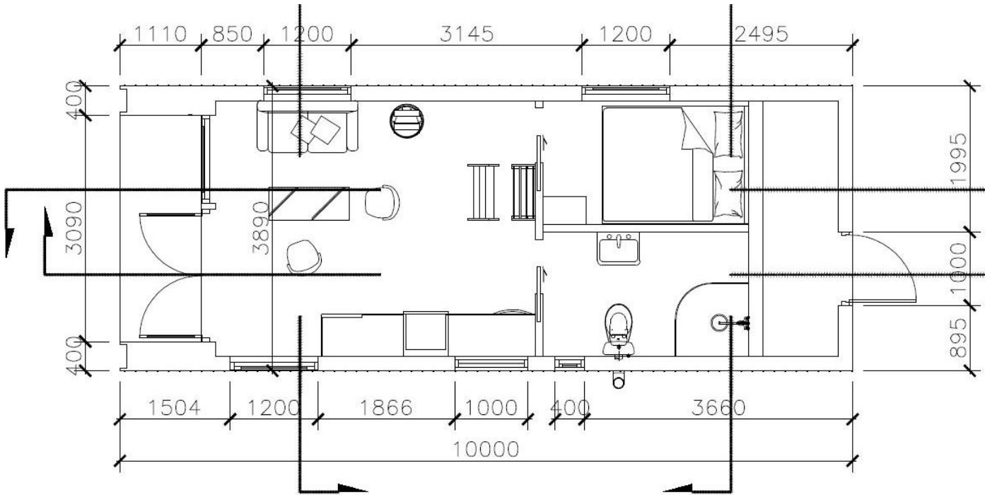
MEZZANINE PLAN SCALE 1: 100
