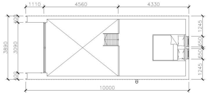
MEZZANINE PLAN SCALE 1: 100
